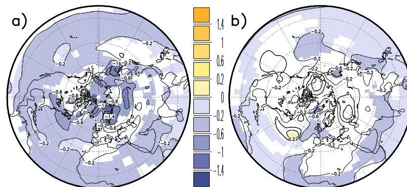
Figure 4. Long-term winter (DJF) ensemble mean difference of near-surface temperature (K) for LMM (1675–1715) minus PI (1715–1790) for (a) simulations EGMAM-1, EGMAM-2, ERIK1, and ERIK2 and (b) four simulations with CCSM3. Colored areas are statistically significant above 99th percentile value based on Student's t test (standard deviation calculated by averaging over variances and degree of freedom is taken as the sum over the individual realizations).
