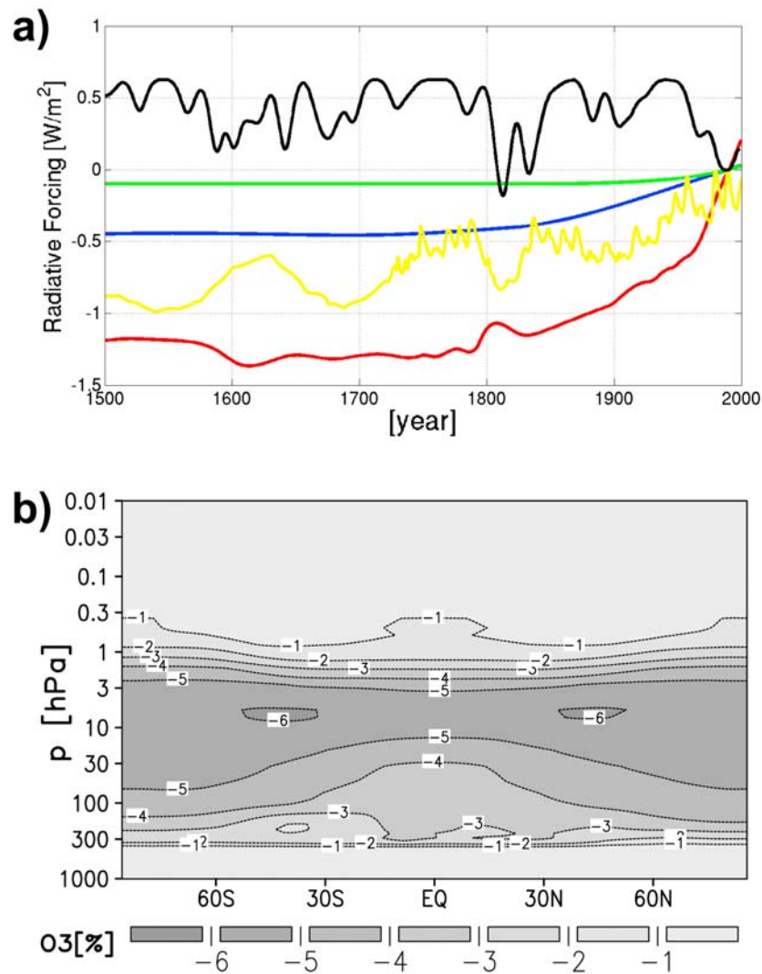
Figure 1. Forcings used to drive the simulations. (a) Solar (yellow), volcanic (black), CO 2 (red), CH 4 (blue), and N 2 O (green) used for EGMAM and ECHO-G. The forcing is represented after conversion to the equivalent radiative forcing assuming the planetary albedo of 0.3 and using the simplified formula given by Ramaswamy et al. [2001, Table 6.2.]. Forcings are referenced to 1990 AD and volcanic forcing is smoothed with a Gaussian-weighted filter to remove fluctuations on time scales less than 30 years. (b) Solar-induced decrease of ozone (volume mixing ratio, percentage change) for Maunder Minimum when compared with present day as applied in EGMAM-2. Forcings for CCSM3 slightly differ from those used for EGMAM and ECHO-G and are shown by Yoshimori et al. [2010].
